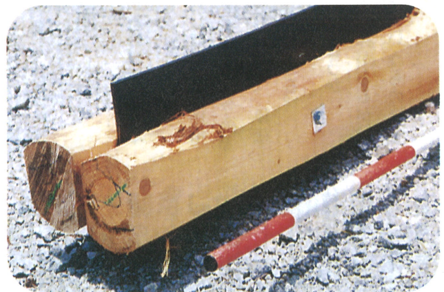
簡易横断溝
